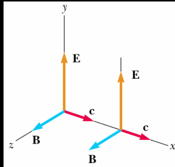
Plane Waves
