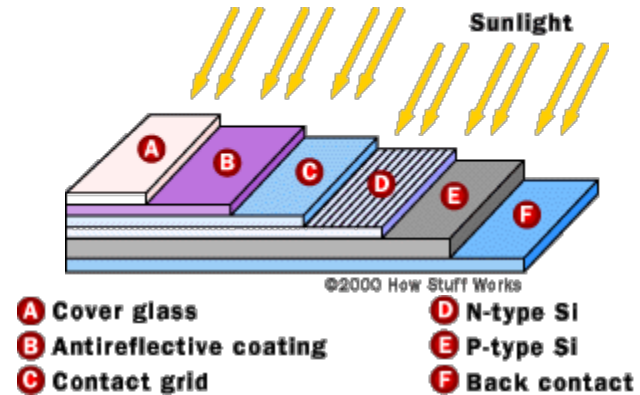
Typical c-Si Solar Cell Structure
