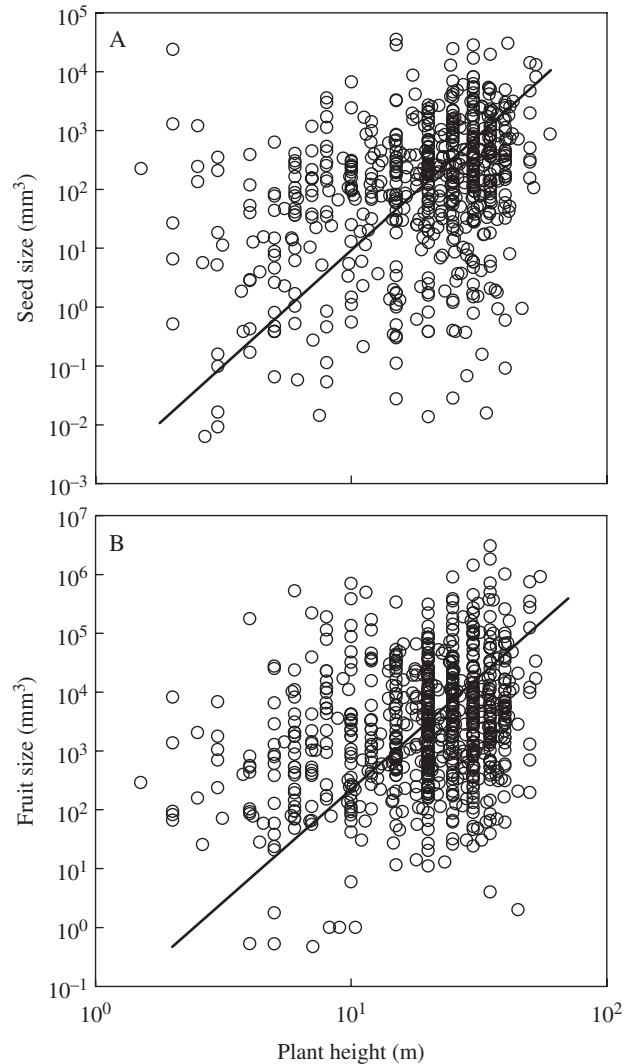
FIG. 2. Relationships between species-mean (A) seed size and plant height, and (B) fruit size and plant height. Correlations statistics are given in Table 3. SMA slopes (and 95 % confidence interval): (A) 3.92 (3.64, 4.22), (B) 3.82 (3.58, 4.08).
