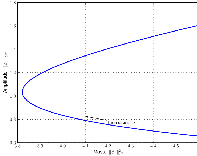
FIGURE 2. A plot of the maximum amplitude with respect to the L^2 norm for a saturated nonlinear Schrödinger equation. Computed at M + 1 = 101 collocation points for \omega \in [0.01, 1.5] .
