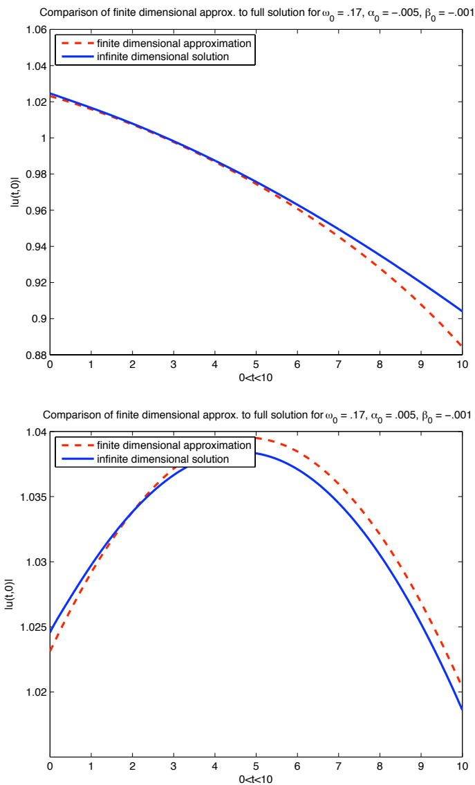
FIGURE 7. A plot of the solution to the system of ODE's as well as the full solution to (1.1) derived for solutions near the minimal soliton for \alpha_0 = \rho_3(0) > 0 and \alpha_0 = \rho_3(0) < 0, \beta_0 = \rho_4(0) < 0 for \omega_0 = .17, N = 500 .
