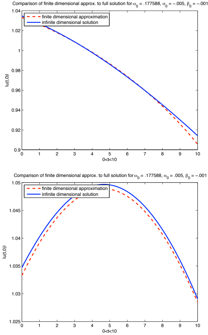
FIGURE 6. A plot of the solution to the system of ODE's as well as the full solution to (1.1) derived for solutions near the minimal soliton for \alpha_0 = \rho_3(0) > 0 and \alpha_0 = \rho_3(0) < 0, \beta_0 = \rho_4(0) < 0 for \omega_0 = .177588, N = 1000 .
