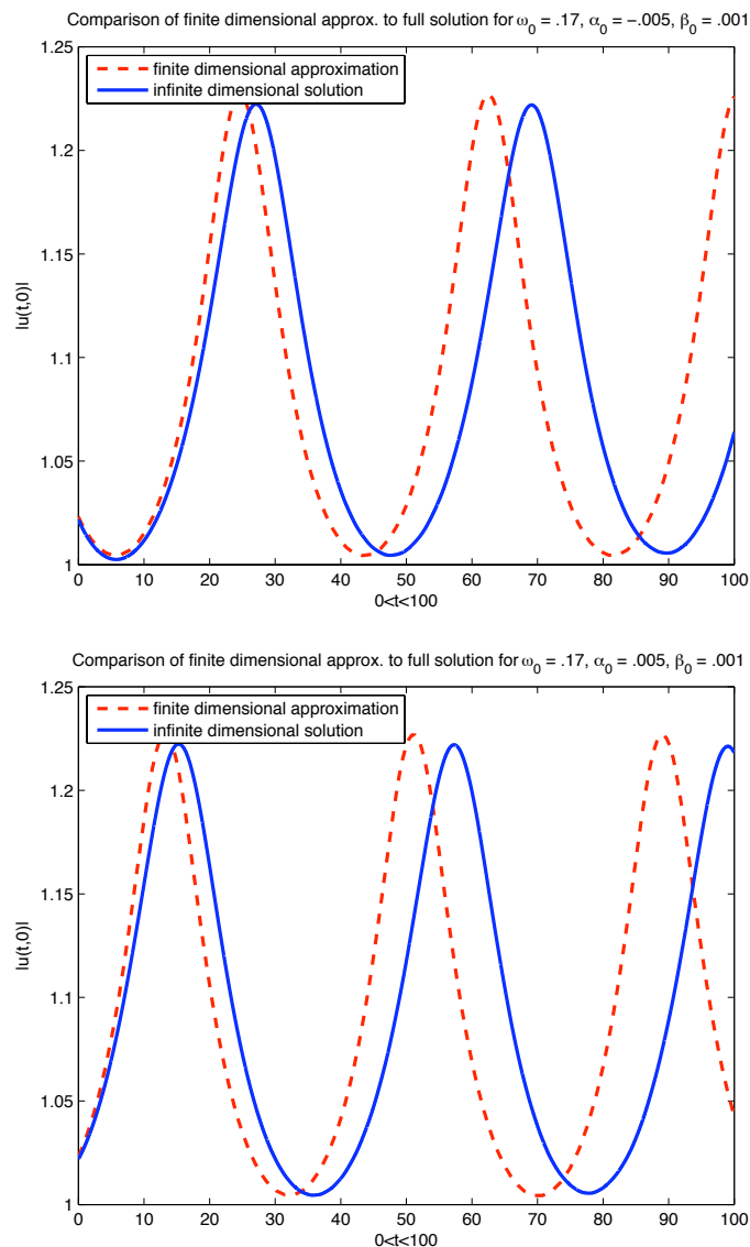
FIGURE 4. A plot of the solution to the system of ODE's as well as the full solution to (1.1) derived for solutions near the minimal soliton for \rho_3(0) > 0 and \rho_3(0) < 0, \rho_4(0) > 0 for \omega_0 = .17, N = 500 .
