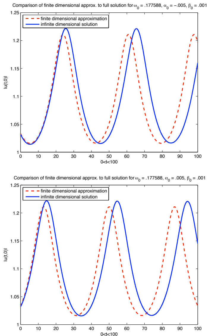
FIGURE 3. A plot of the solution to the system of ODE's as well as the full solution to (1.1) derived for solutions near the minimal soliton for \rho_3(0) > 0 and \rho_3(0) < 0, \rho_4(0) > 0 for \omega_0 = .177588, N = 1000 .
