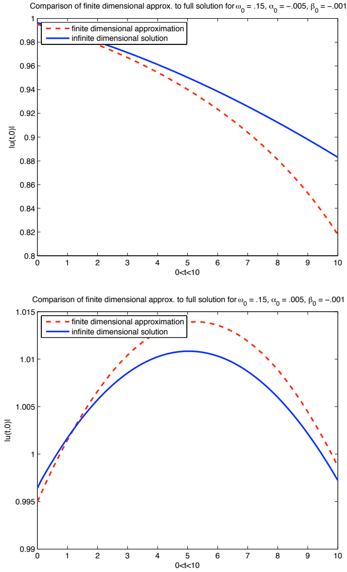
FIGURE 8. A plot of the solution to the system of ODE's as well as the full solution to (1.1) derived for solutions near the minimal soliton for \alpha_0 = \rho_3(0) > 0 and \alpha_0 = \rho_3(0) < 0, \beta_0 = \rho_4(0) < 0 for \omega_0 = .15, N = 500 .
