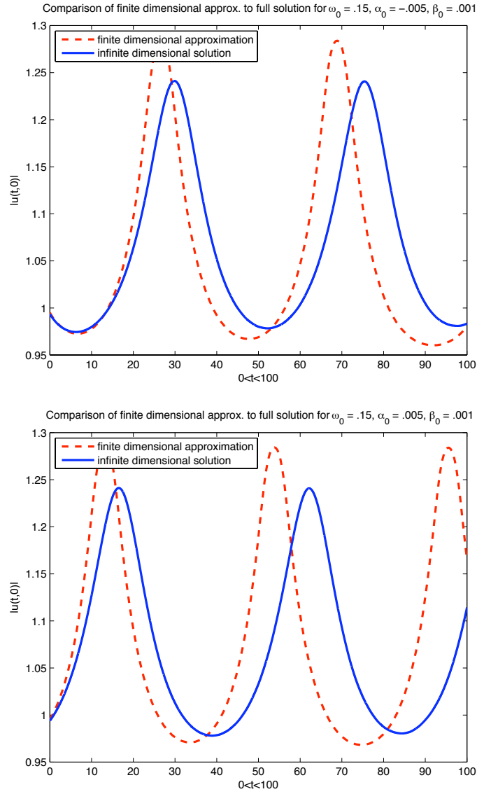
FIGURE 5. A plot of the solution to the system of ODE's as well as the full solution to (1.1) derived for solutions near the minimal soliton for \alpha_0 = \rho_3(0) > 0 and \alpha_0 = \rho_3(0) < 0 , \beta_0 = \rho_4(0) > 0 for \omega_0 = .15 , N = 500 .
