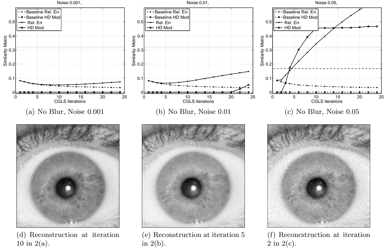
Figure 2. Reconstruction of simulated well-focused low-resolution iris data containing increasing amounts of noise. Dotted line at 0.32: HD matching cutoff. Dash-dot line: HD of reference low-resolution image (noise=0.001: HD(ref)=0, noise=0.01: HD(ref)=0, noise=0.05: HD(ref)=0.17).
