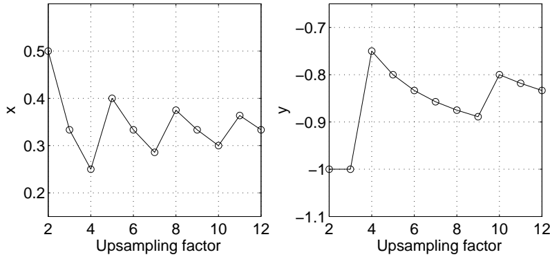
Figure 6. Convergence of \Delta p and \Delta q with upsampling factor r .
