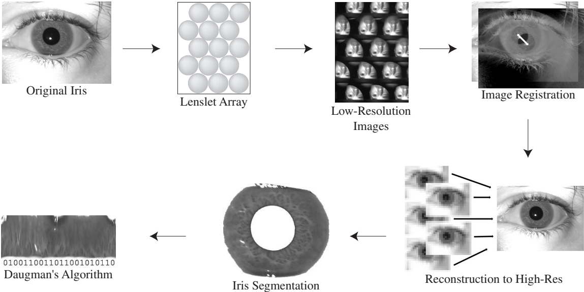
Figure 1. A visual overview of the reconstruction process.
