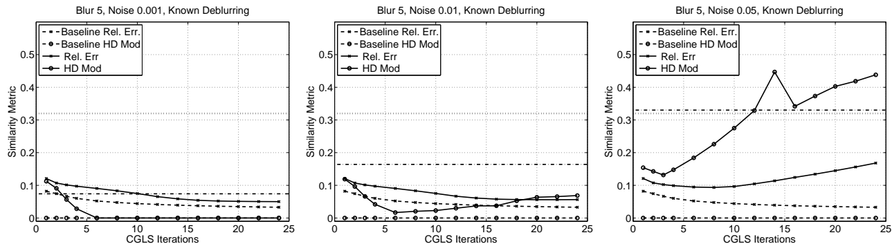
(a) Gaussian blur \sigma = 5 , Noise 0.001, (b) Gaussian blur \sigma = 5 , Noise 0.01, (c) Gaussian blur \sigma = 5 , Noise 0.05, Known Blur
