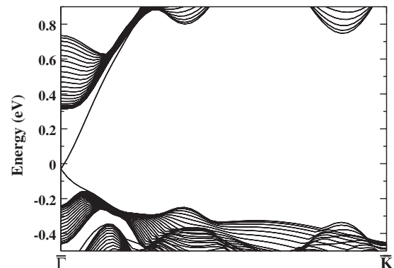
FIG. 30. Wannier-interpolated energy bands of a freestanding (111)-oriented slab containing 25 quintuple layers of Bi 2 Se 3 plotted along the \bar{\Gamma} - \bar{K} line in the surface Brillouin zone. A pair of topologically protected surface bands can be seen emerging from the dense set of projected valence and conduction bulklike bands and crossing at the time-reversal-invariant point \bar{\Gamma} . Adapted from Zhang et al. , 2010.
