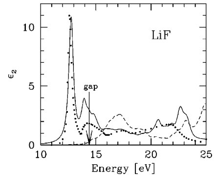
FIG. 9. Calculated optical absorption spectrum of LiF with (solid lines) and without (dashed lines) electron-hole interaction, using three valence bands, six conduction bands, 500 \mathbf{k} points in the BZ, and an artificial broadening of 0.25 eV. The experimental data (●) are from Ref. 36.
