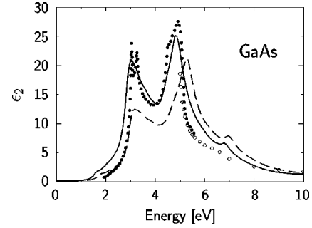
FIG. 6. Calculated optical absorption spectrum of GaAs with (solid lines) and without (dashed lines) electron-hole interaction, using three valence bands, six conduction bands, 500 \mathbf{k} points in the BZ, and an artificial broadening of 0.15 eV. The dots denote experimental data from Ref. 32 (○) and Ref. 33 (●).
