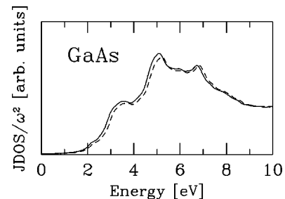
FIG. 7. Density of excited states for GaAs divided by \omega^2 (in arbitrary units). The dashed line corresponds to vertical band-to-band transitions while the solid line results from the BSE, including the electron-hole interaction.
