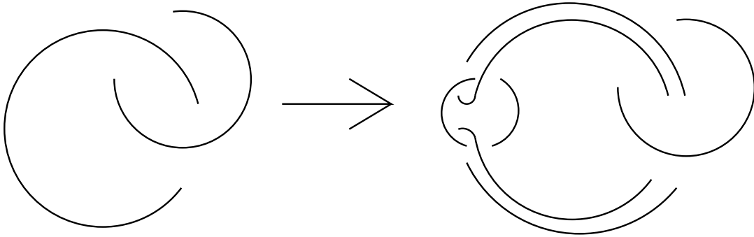
Figure 2: The Bing double of the Hopf link yields a Brunnian Link with planar components
