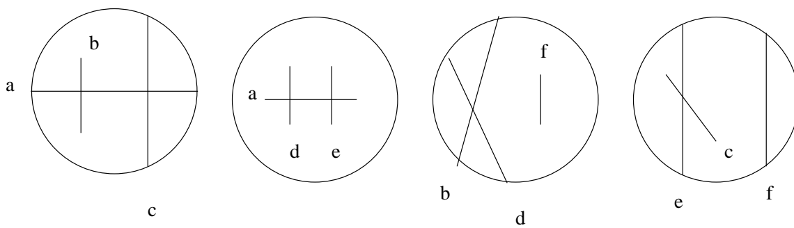
Figure 6: Diagrams for two triple points.
