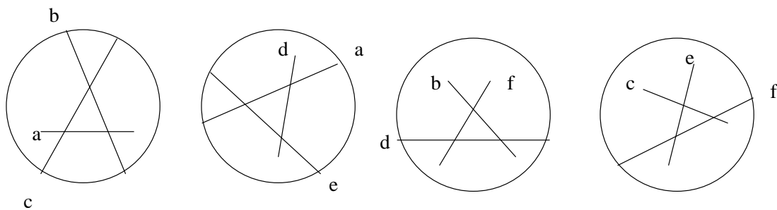
Figure 8: Diagrams for four triple points.
