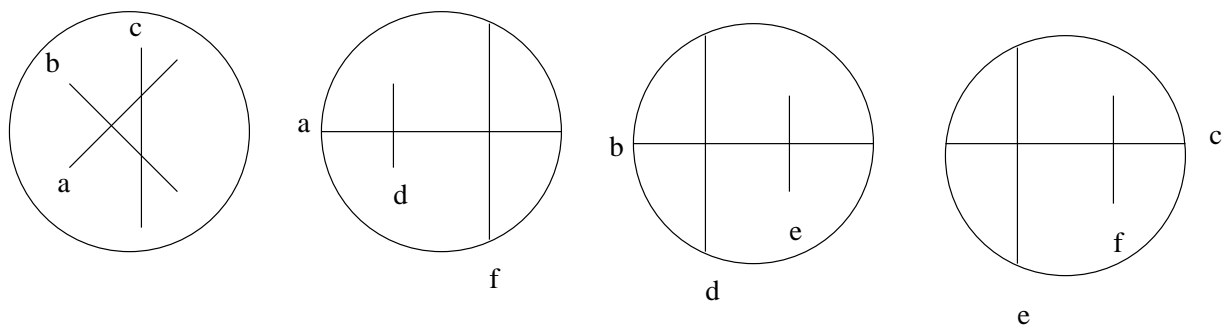
Figure 7: Diagrams for three triple points.
