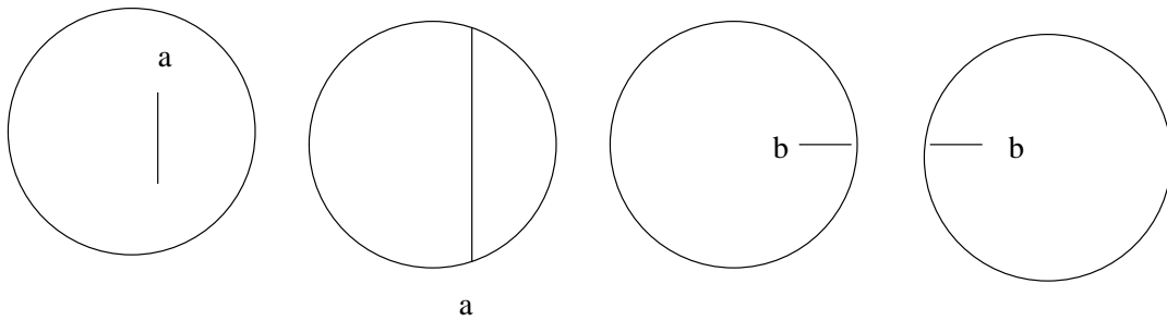
Figure 4: An abstract picture of a ribbon and a clasp singularity. The first disk corresponds to the interior arc from the ribbon singularity, the second, the exterior arc. The third and fourth disks have the clasp singularities drawn.
