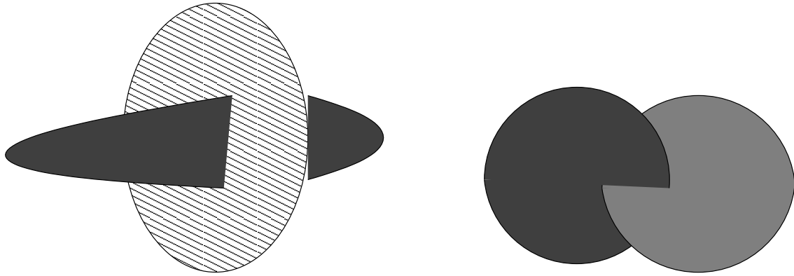
Figure 3: A ribbon singularity and a clasp singularity
