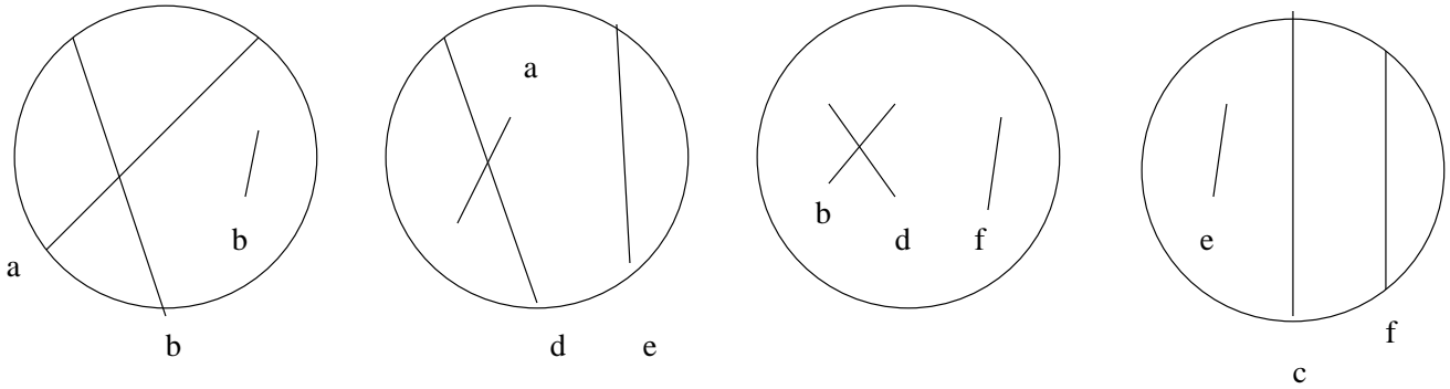
Figure 5: Diagrams for one triple point. \Delta_1 is on the left \Delta_2 to its right, \Delta_3 the third disk, and \Delta_4 is on the right.
