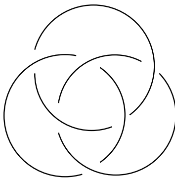
Figure 1: The Borromean Rings pictured here appear to be made out of circles
