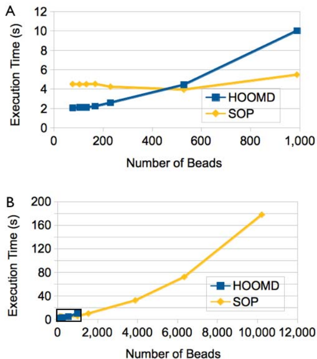
Fig. 7. Execution times comparisons with HOOMD. (A) Comparison of execution times of the SOP Model implemented in our MD simulation code as compared to the SOP model implemented in HOOMD for system sizes up to \sim 1,000 beads, which was the maximum hardware limit on the NVIDIA Tesla C2070. (B) The same comparison for systems sizes up to \sim 10,000 beads, which is the maximum hard limit for our simulation code on the NVIDIA Tesla C2070.
