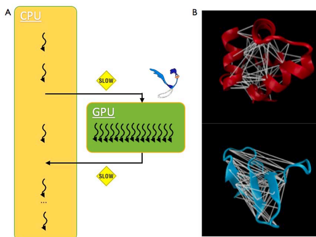
Fig. 1. MD simulations of biomolecular systems on GPUs. (A) A schematic of the processing flow of CPUs and GPUs. In a single-core processor, a single thread sequentially executes commands while GPUs have many threads that executes commands in parallel. (B) A cartoon of two typical proteins with the native interactions between residues shown. Each interaction can be computed independently in MD simulations, which makes GPUs ideal architectures for implementation of MD simulation algorithms.
