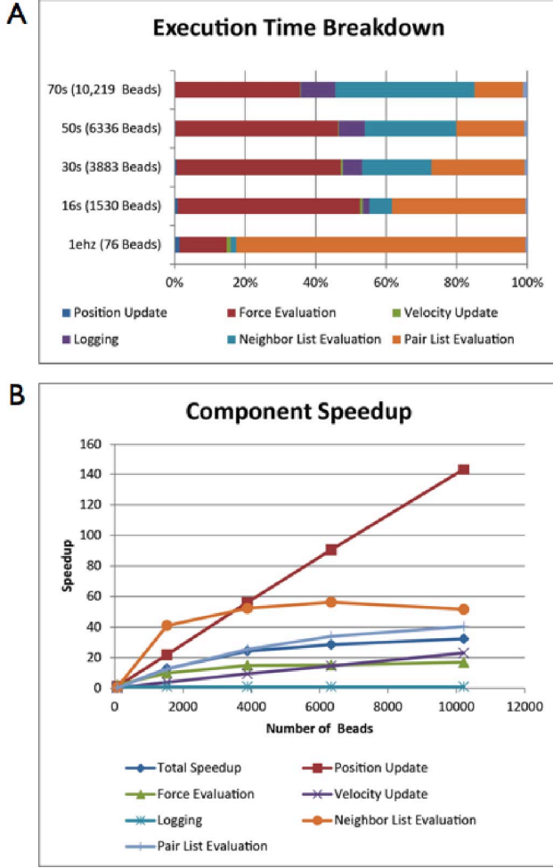
Fig. 6. Relative execution times and speedup of different components of the SOP model MD simulations with the parallel neighbor list algorithm. (A) The percentages of the execution times are shown for different components of the GPU-optimized MD simulations for the biologically relevant systems we simulated. (B) The speedup of the different components of the GPU-optimized MD simulations are shown for the same biologically relevant systems as compared to the equivalent single-core CPU-optimized MD simulations.
