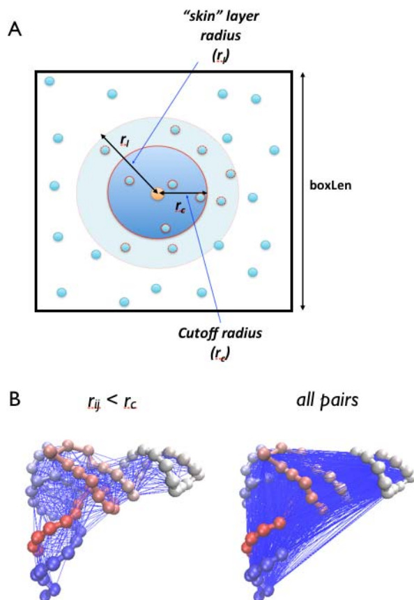
Fig. 4. Original Verlet neighbor list algorithm (A) In the Verlet neighbor list algorithm, out of a master list of all pairs of possible interactions, a neighbor list is constructed of interactions within a "skin" layer radius ( r_l ) distance cutoff. The neighbor list is updated every n timesteps from which a pair list is constructed of interactions within a cutoff radius ( r_c ) distance cutoff. At every timestep, the forces are evaluated only for the members of the pair list. (B) The structure of tRNA Phe is shown with blue lines indicating members of the pair list (left) and all possible interaction pairs (right).
