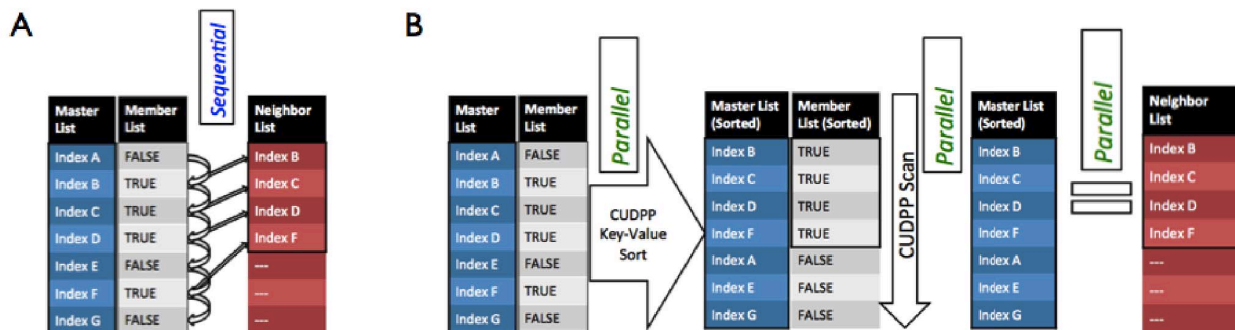
Fig. 5. Sequential and parallel Verlet neighbor list algorithms. (A) A schematic of the original Verlet neighbor list algorithm that involves an inferentially sequential implementation. (B) A parallel neighbor list algorithm that is specifically optimized for GPUs that involves only parallel operations.
