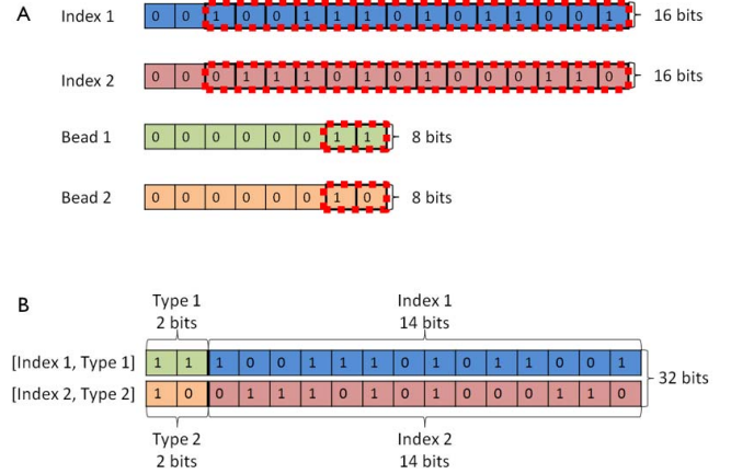
Fig. 2. Schematic of the type compression optimization for representing the indices and types of the interacting beads. (A) A total of 48 bits are required when using two 16-bit ushorts and two 8-bit uchar to represent two interaction indices and two interaction types. A total of 16 bits will always be unused. The bits that will be used in the compressed type is highlighted in red. (B) Only 32 bits are required when using a single 32-bit ushort to represent two interaction indices and two interaction types. Note that there are no unused bits when simulating the 70s ribosome (10,219 beads).
